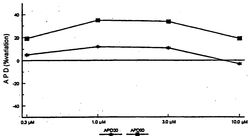
Effect of compound of example 1 on action potential duration (APD) recorded in guinea-pig papillary muscle. Action potential duration was measured at 30% (APD30) and 90% (APD90) of repolarization.
